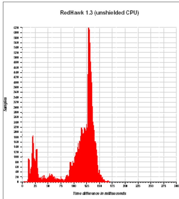
FIGURE 3: RedHawk 1.3 Unshielded CPU Results
