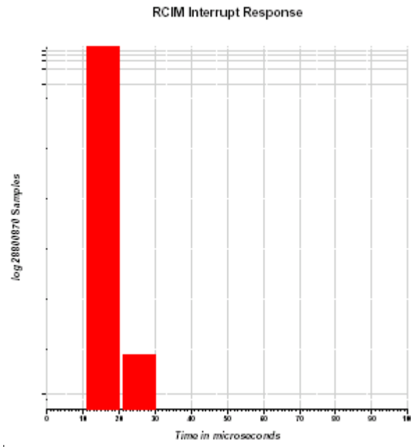
FIGURE 7: RCIM Interrupt Response Results
