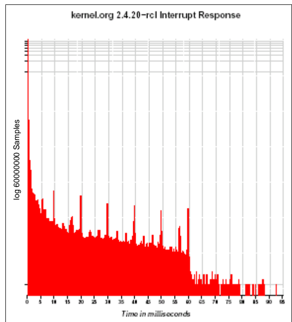
FIGURE 5: kernel.org 2.4.20-rc1 Interrupt Response Results
